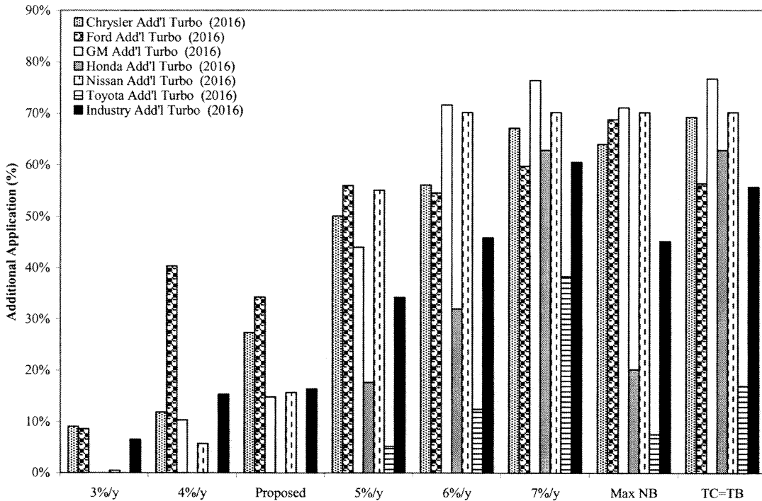
Figure IV.F.10. Additional Application of Engine Turbocharging & Downsizing (MY 2016)
