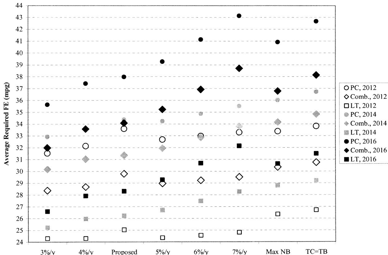
Figure IV.F.8. Average Required Fuel Economy (MYs 2012, 2014, and 2016)
