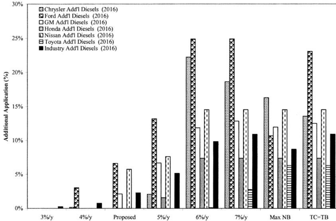
Figure IV.F.11. Additional Application of Diesel Engines (MY 2016)
