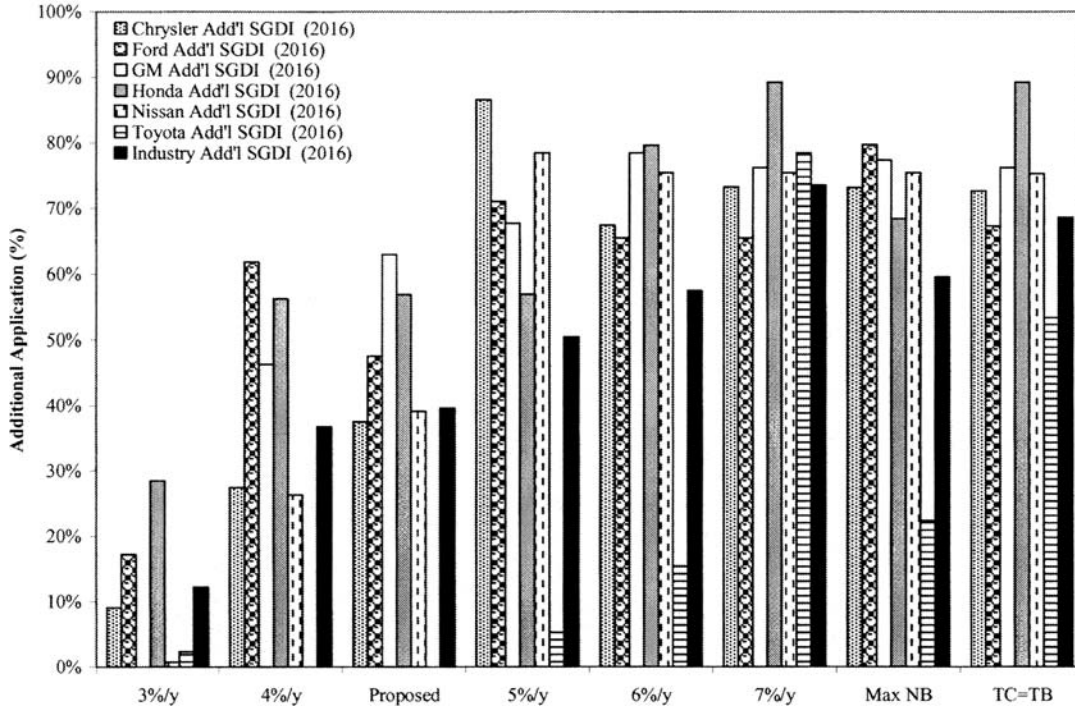
Figure IV.F.9. Additional Application of GDI (MY 2016)
